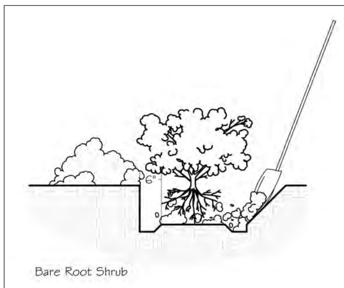
Fig. 5.11. Backfilling the hole. (Source: Robert Schutzki; graphics by Kristin Faasse.)
