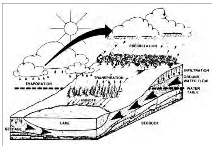
Figure 1.2. Precipitation pathways to inland lakes. (Source: Lake and Reservoir Restoration Guidance Manual , [1st ed.].)
