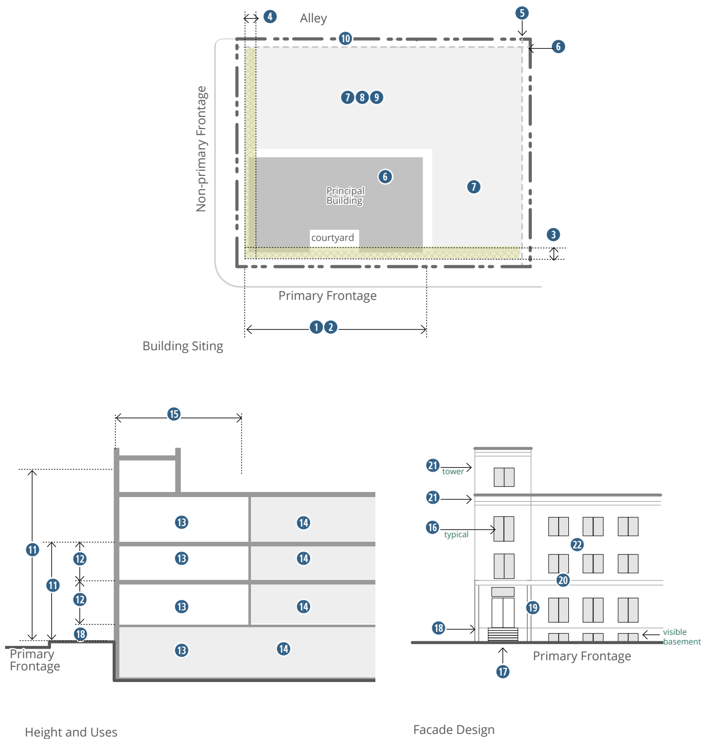
Figure 3-11. General Building
