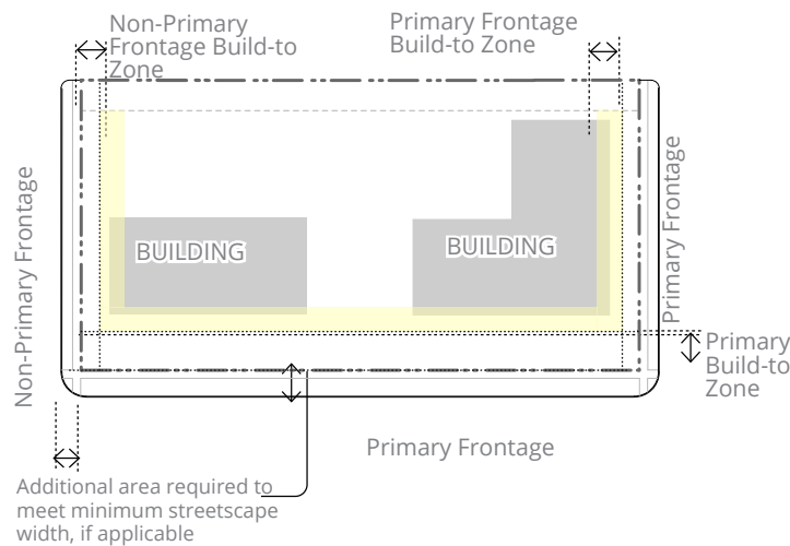
Figure 18-2. Build-to Zones
