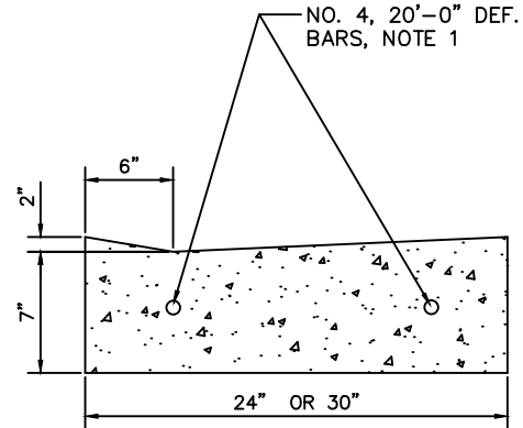
GUTTER
