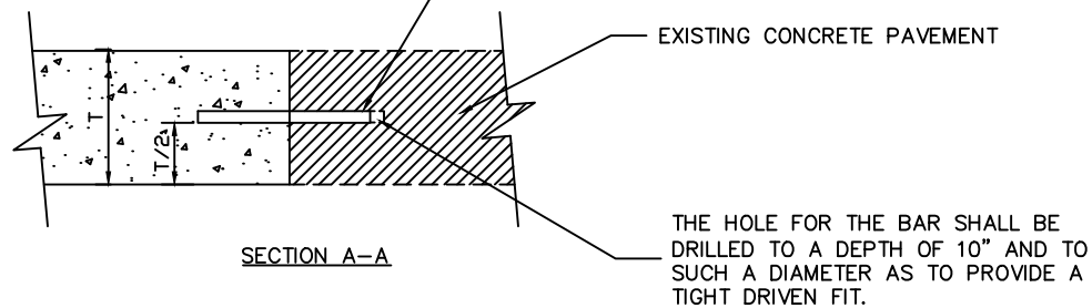
PAVEMENT TIES EXISTING PAVEMENT
