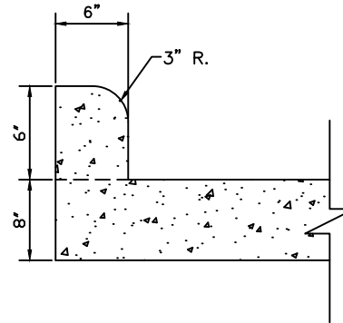
INTEGRAL CURB
