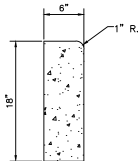
CURB
