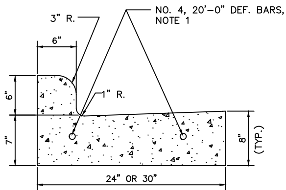
CURB AND GUTTER
