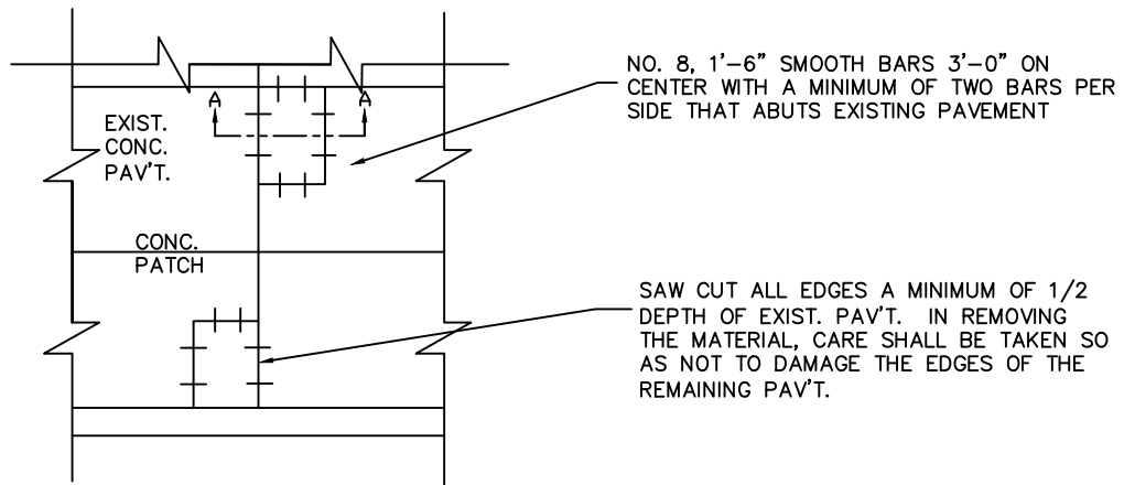
PAVEMENT TIES CONCRETE PATCHING
