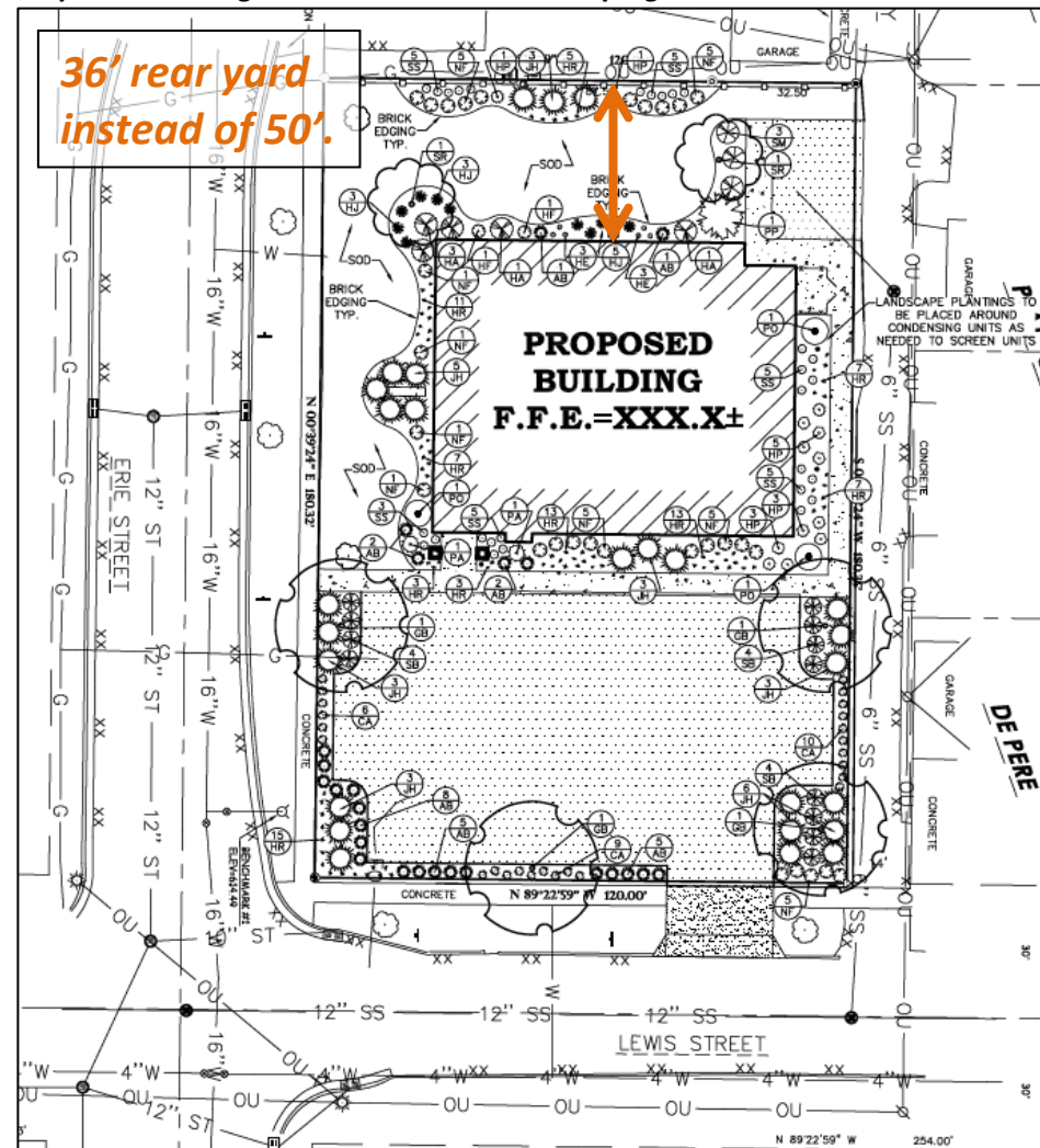
Proposed building rear setback with landscaping shown.
